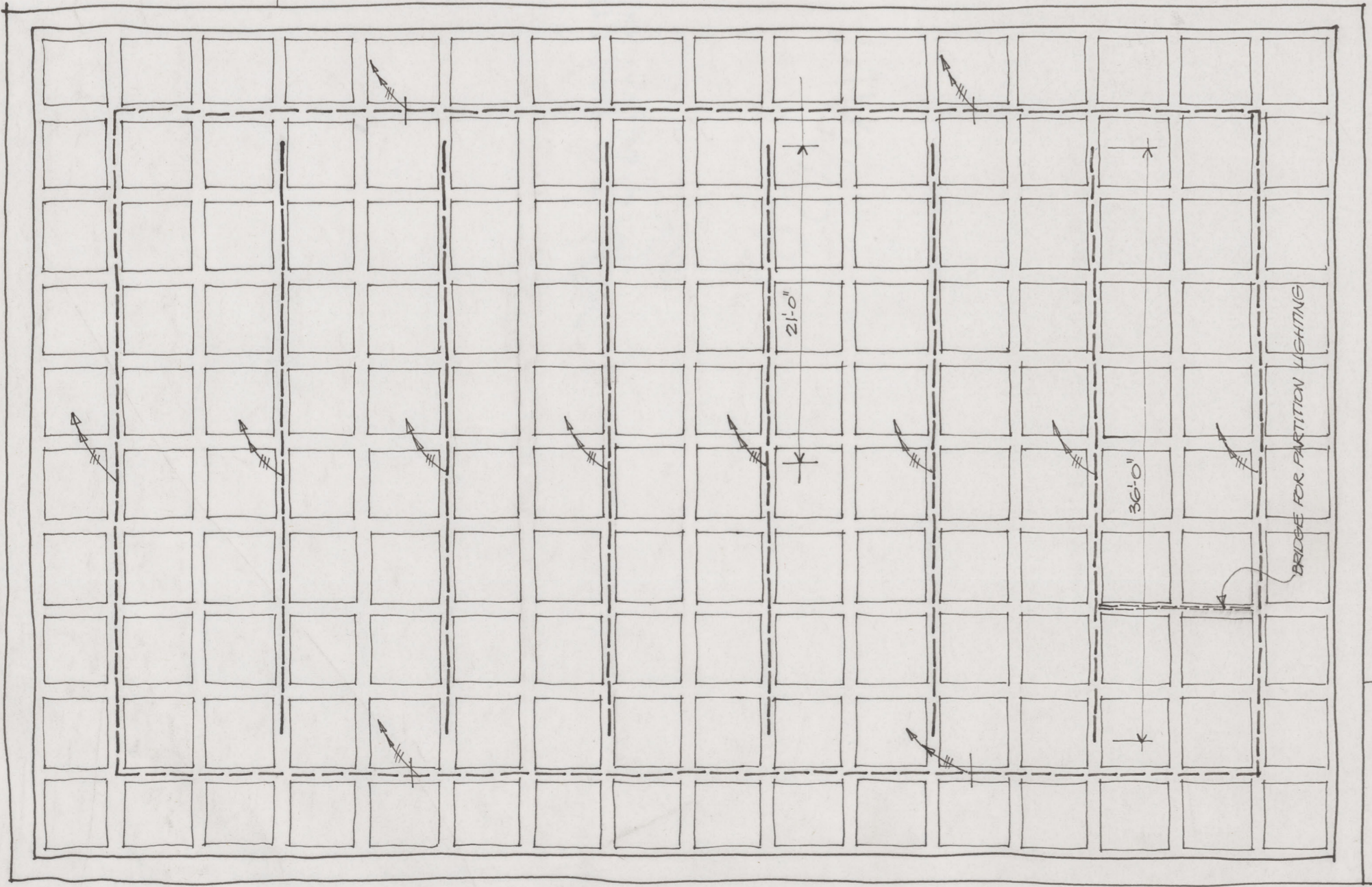
TYPICAL GALLERY REFLECTED CEILING PLAN
