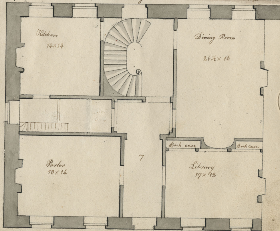
First Story
