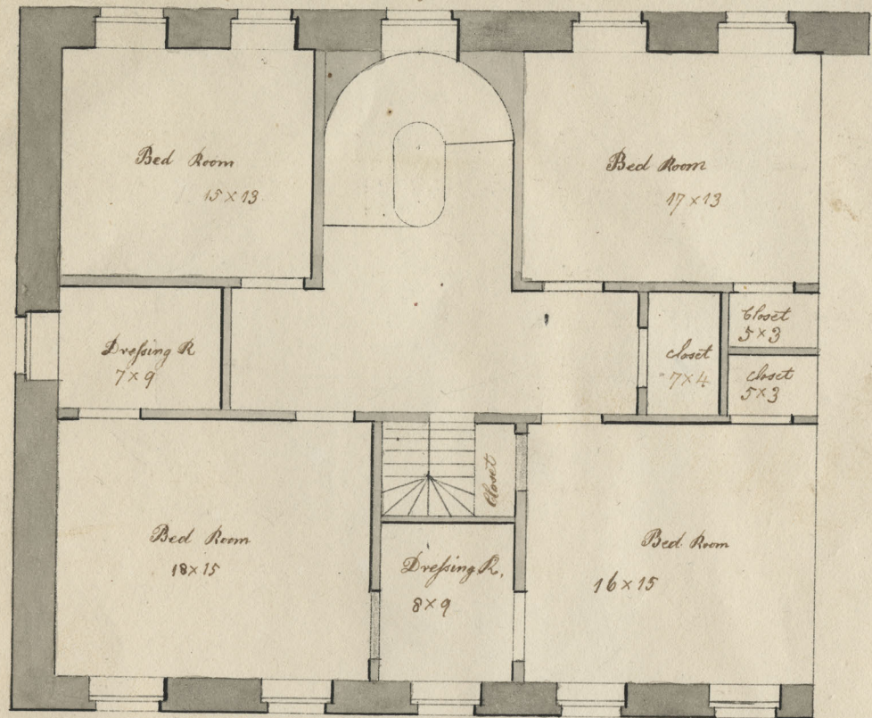
Third Story
