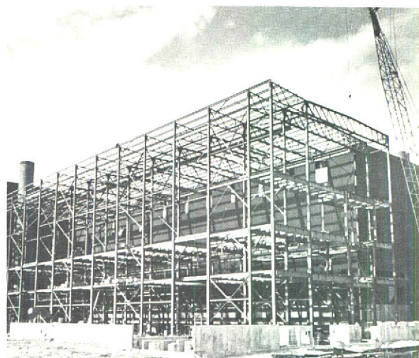
Over 7,000 tons of structural steel were fabricated and erected by Central Bridge for this iron ore pelletizing plant in Labrador.
