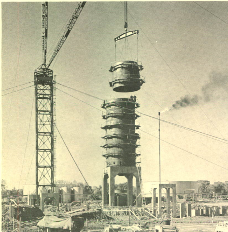
5. First reactor regenerator and stripper of its kind built in Canada for the petroleum industry was fabricated and field erected by the Plate Fabrication Division.
