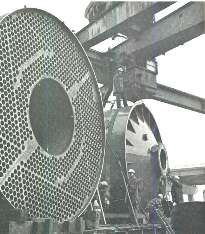
1. Two huge vacuum pans used for refining sugar are readied for shipment by TIW's Plate Fabrication Division.
