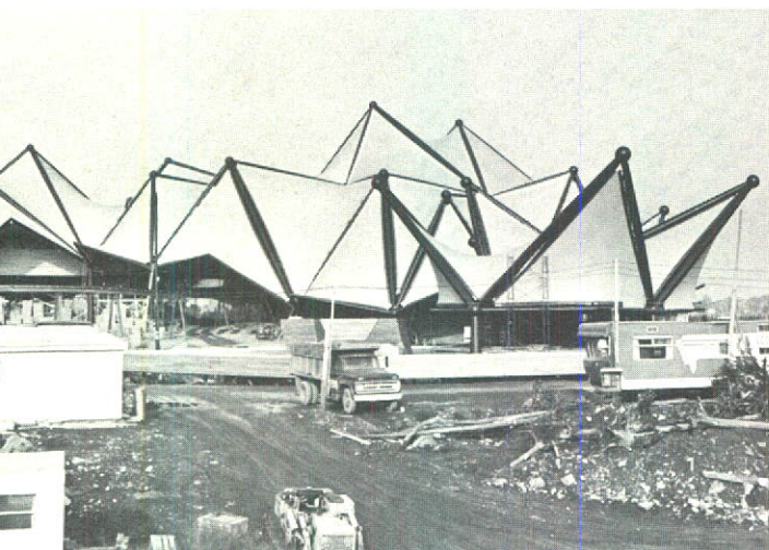
TIW's Central Bridge Division fabricated and erected the unique steel frame supporting Ontario's Expo '67 Pavilion and also installed the fiber glass roofing material.
