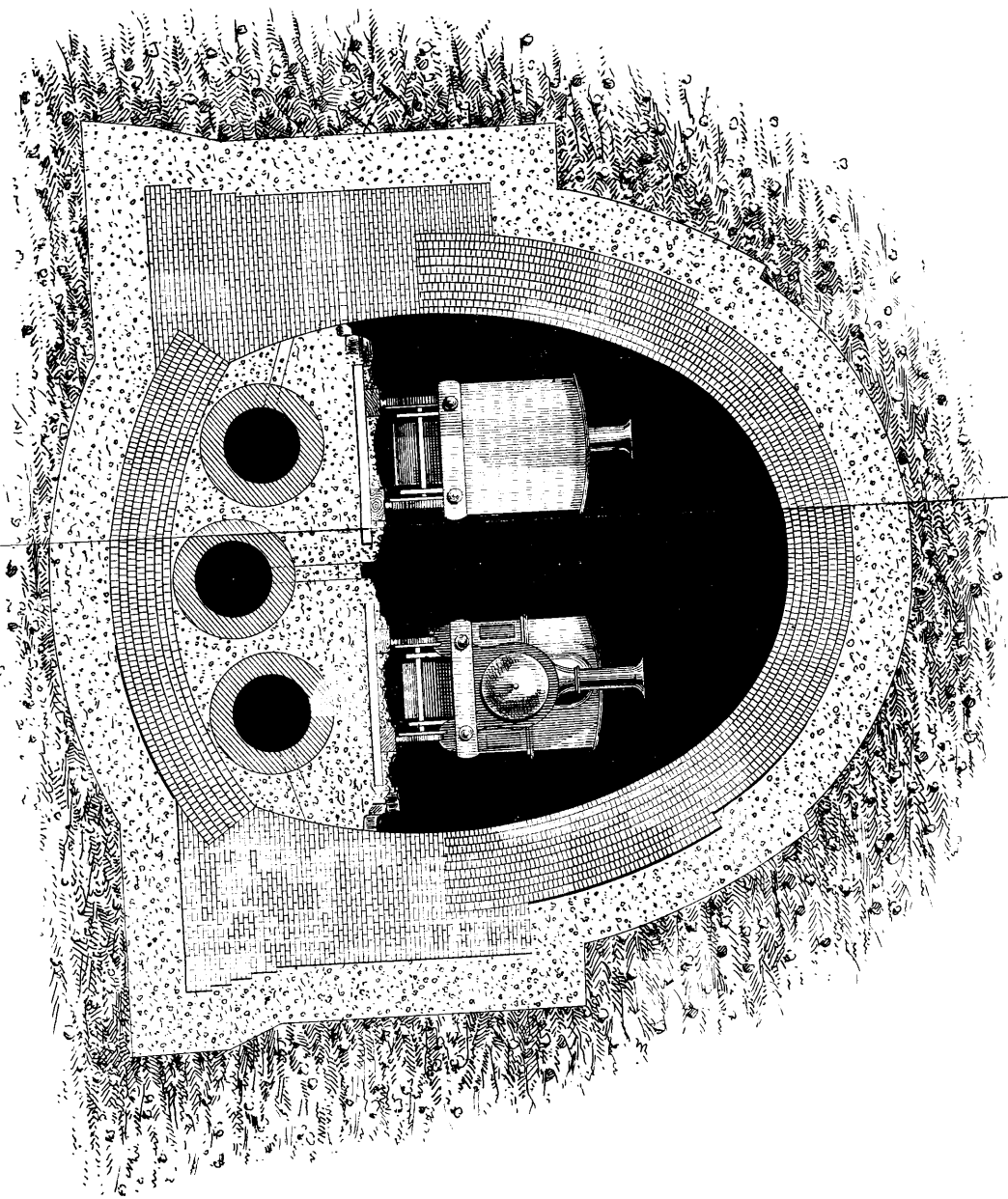
SECTION OF CHANNEL RAILWAY TUNNEL AS PROPOSED BY MR. GEO. REMINGTON C.E.
