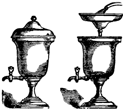
LOYSEL'S HYDROSTATIC URN.
