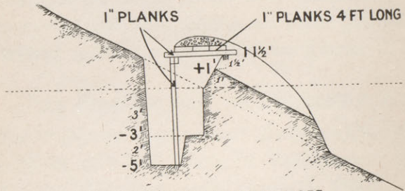
SECTION OF TRENCH ON A STEEP SLOPE
