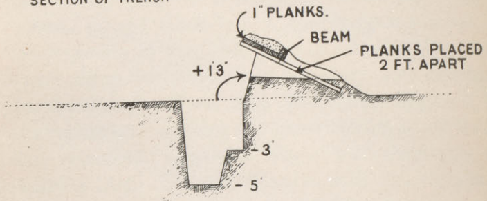
SECTION OF TRENCH
