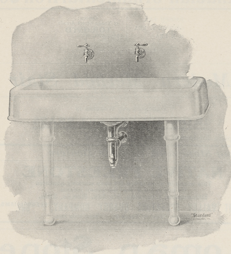
"Standard" PLATE P 1245.—Porcelain Enameled Sink, with Apron all around, Enameled Sink Legs with Wall Supports, Nickel-plated Strainer, Fuller adjustable Flange Bibbs and "P" Trap with Waste and Vent to Wall.
