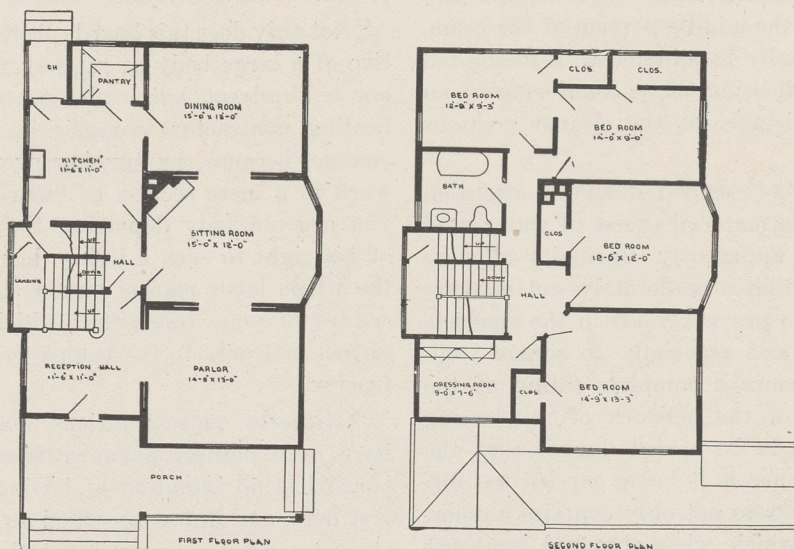
PLANS OF DESIGN FOR MODERATE COST HOUSE.
