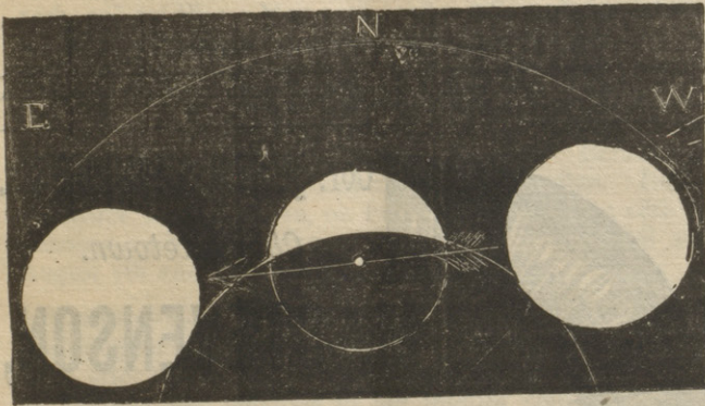
(The arrow marks the course of the Moon's centre across the Earth's Shadow; the outer circle shows the limit of the Penumbra.)
