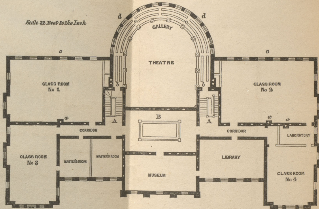
SECOND FLOOR—NORMAL SCHOOL BUILDING.
