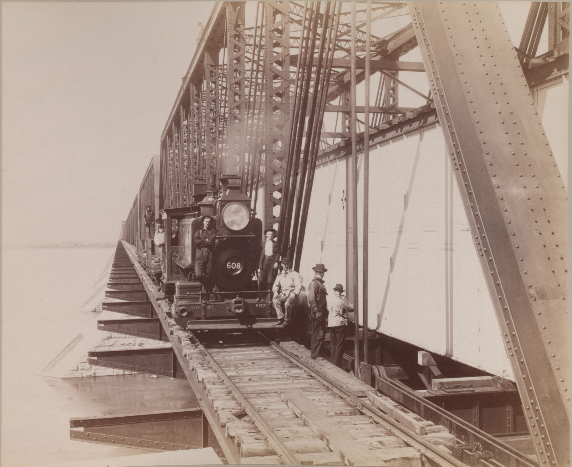
— Temporary Track On Extended Floor Beams — — Shewing Service Locomotive —
